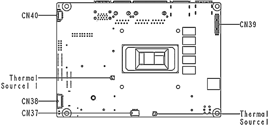
Bottom View
